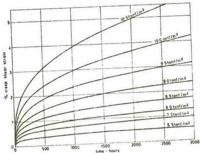
FIG. 10 MODIFIED TORSION CREEP CURVES (0.18 PERCENT CARBON STEEL AT 400°C)
